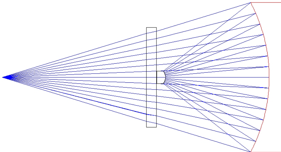
Figure 3 - Null testing concave ellipse at conic foci
