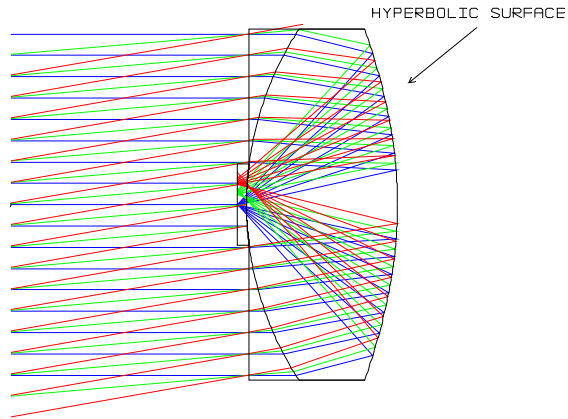
Figure 5 - Hyperbolic collection lens for laser target designator (as used)
