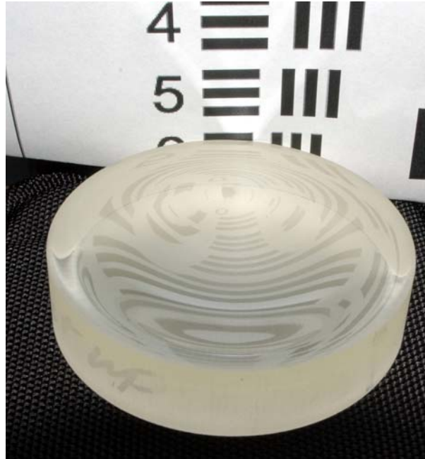
Figure 8 - Aspheric surface with 950 microns departure over 45 mm
