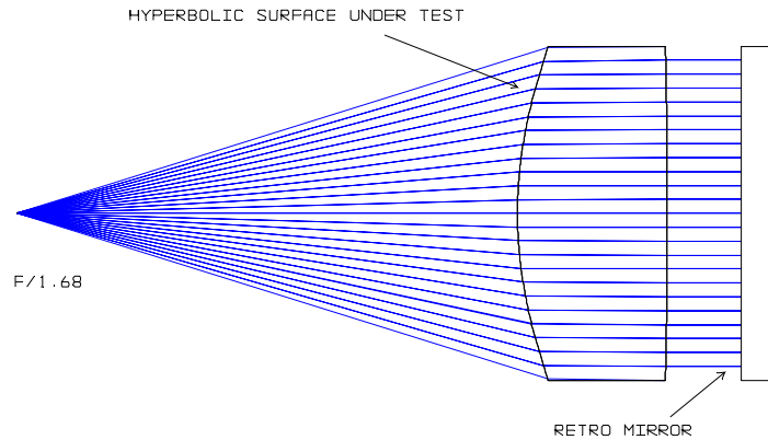
Figure 6 - Testing the same hyperbolic surface in transmission at 632.8 nm as a collimating lens
