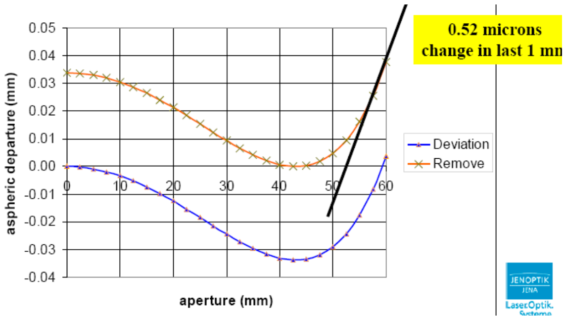
Figure 7 - Slope of the aspheric departure often determines manufacturability
