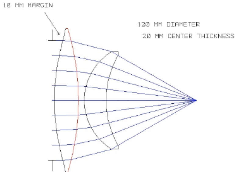
Figure 9 - Allow 10 mm on the radius for aspheric polishing
