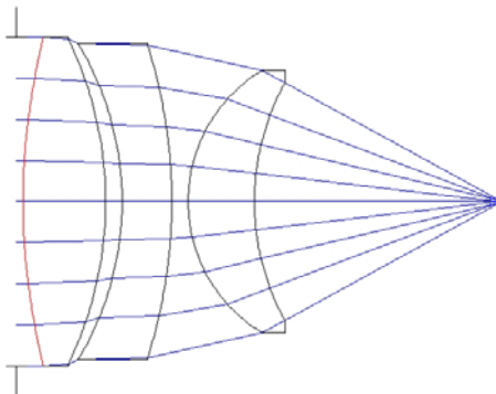
Figure 2 – Three element f/1 transmission sphere example
