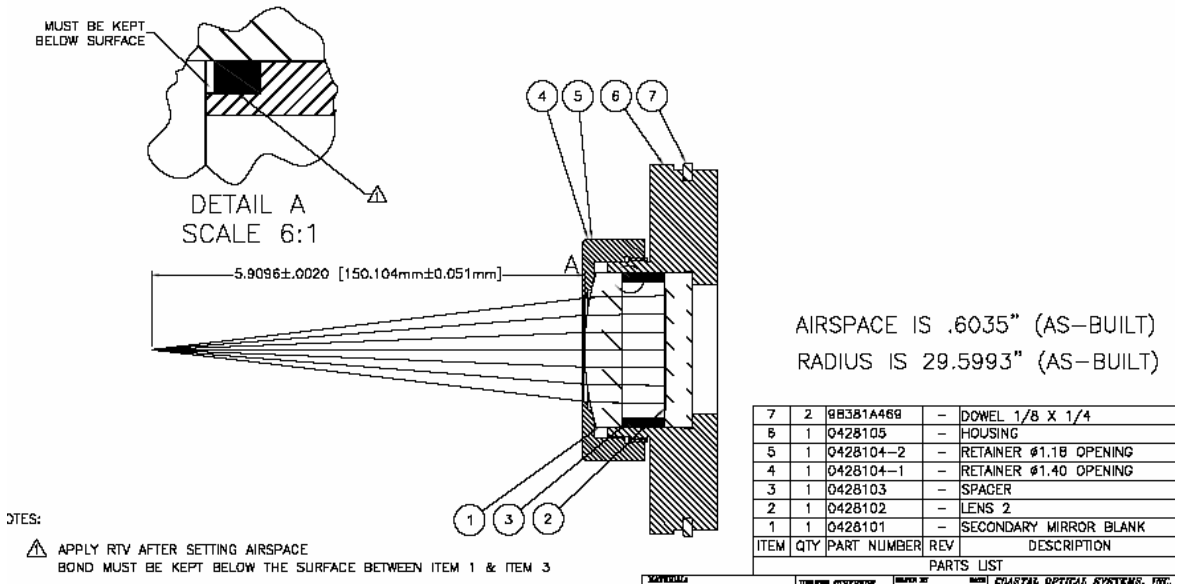
Figure 4 - Testing a convex hyperbolic secondary mirror in transmission
