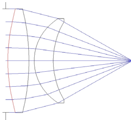
Figure 1 - 2 element f/1 transmission sphere
